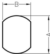
MOUNTING HOLE CHASSIS THICKNESS F
