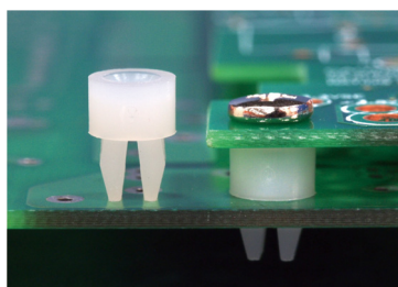
MOUNTING HOLE THICKNESS 2.4
