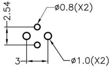
MOUNTING HOLES
