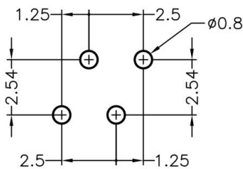
RECOMMEND MOUNTING HOLE
